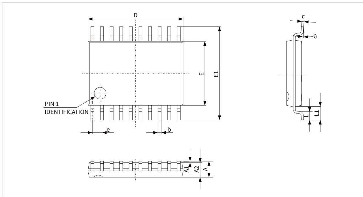
Figure 8-3 TSSOP20 outline
