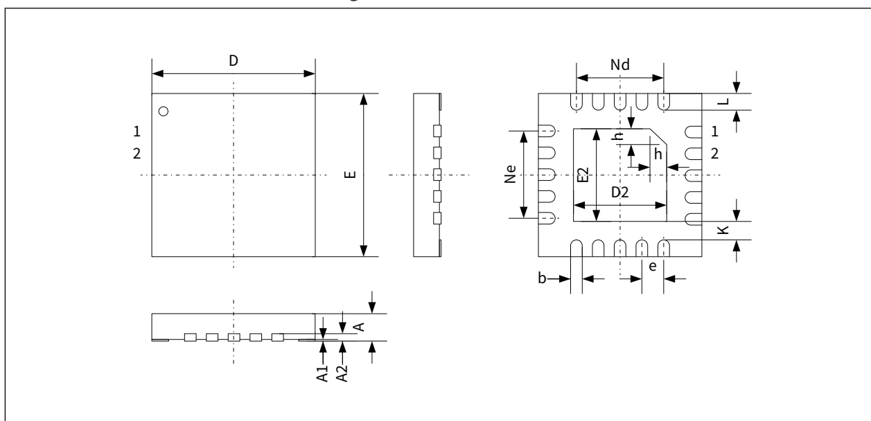
Figure 8-5 QFN20 outline
