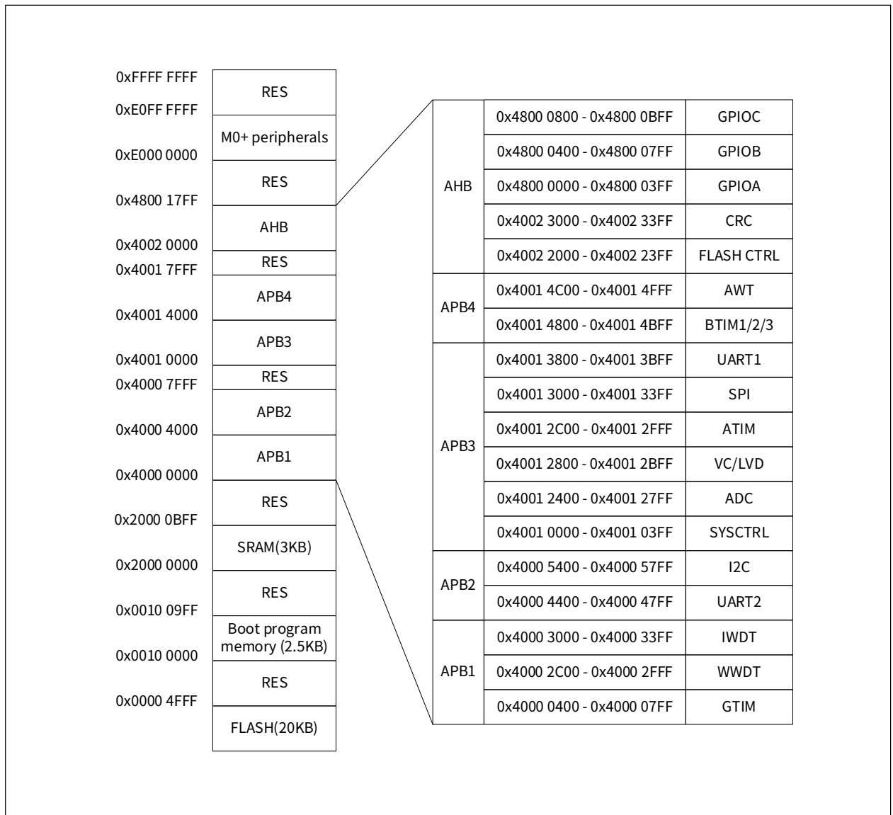
Figure 6-1 CW32F003x3/x4 internal address mapping
