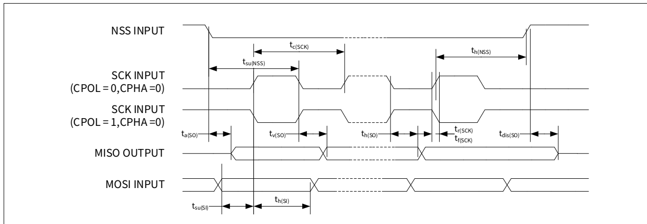
Figure 7-10 SPI timing diagram - slave mode and CPHA=1
