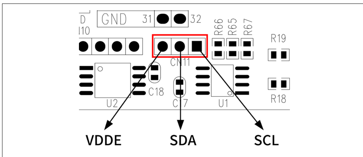
Figure 6-6 CN11 pin definition
