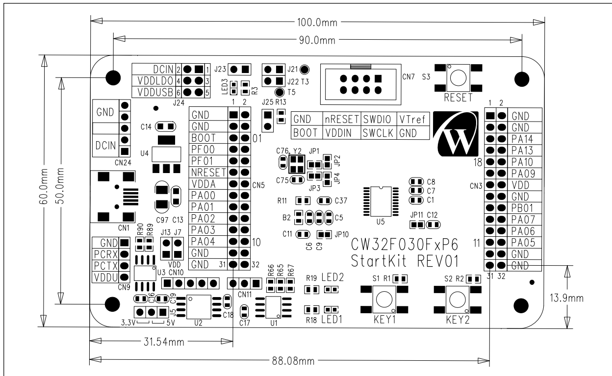
Figure 6-2 CW32F030FxPx StartKit Mechanical Dimensions
