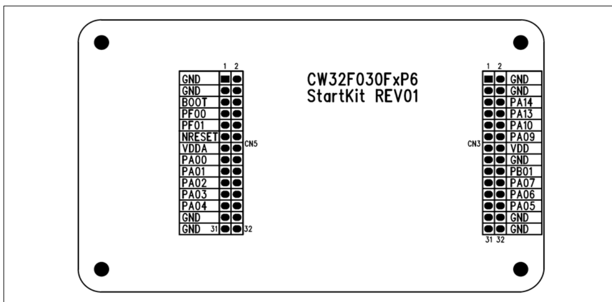
Figure 6-4 Expansion interface layout
