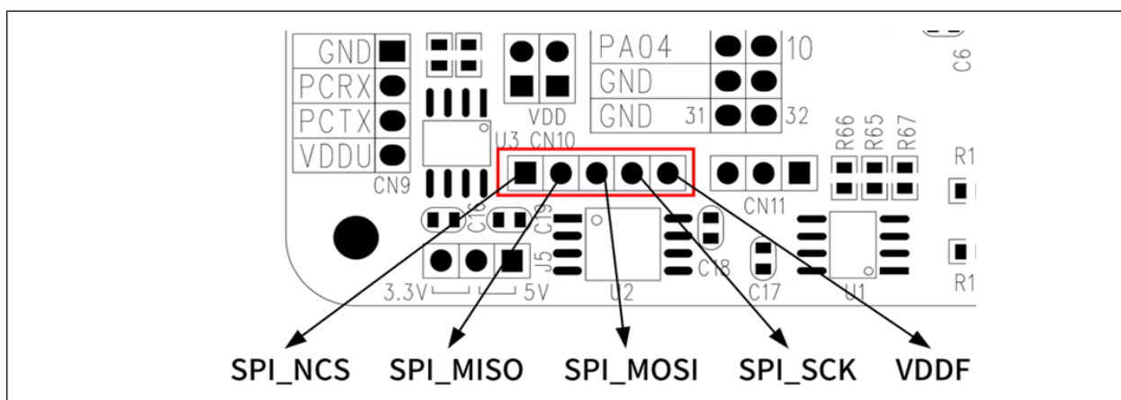
Figure 6-5 CN10 pin definition
