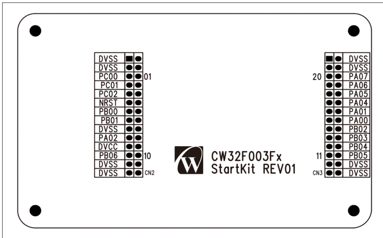
Figure 6-4 Expansion interface layout
