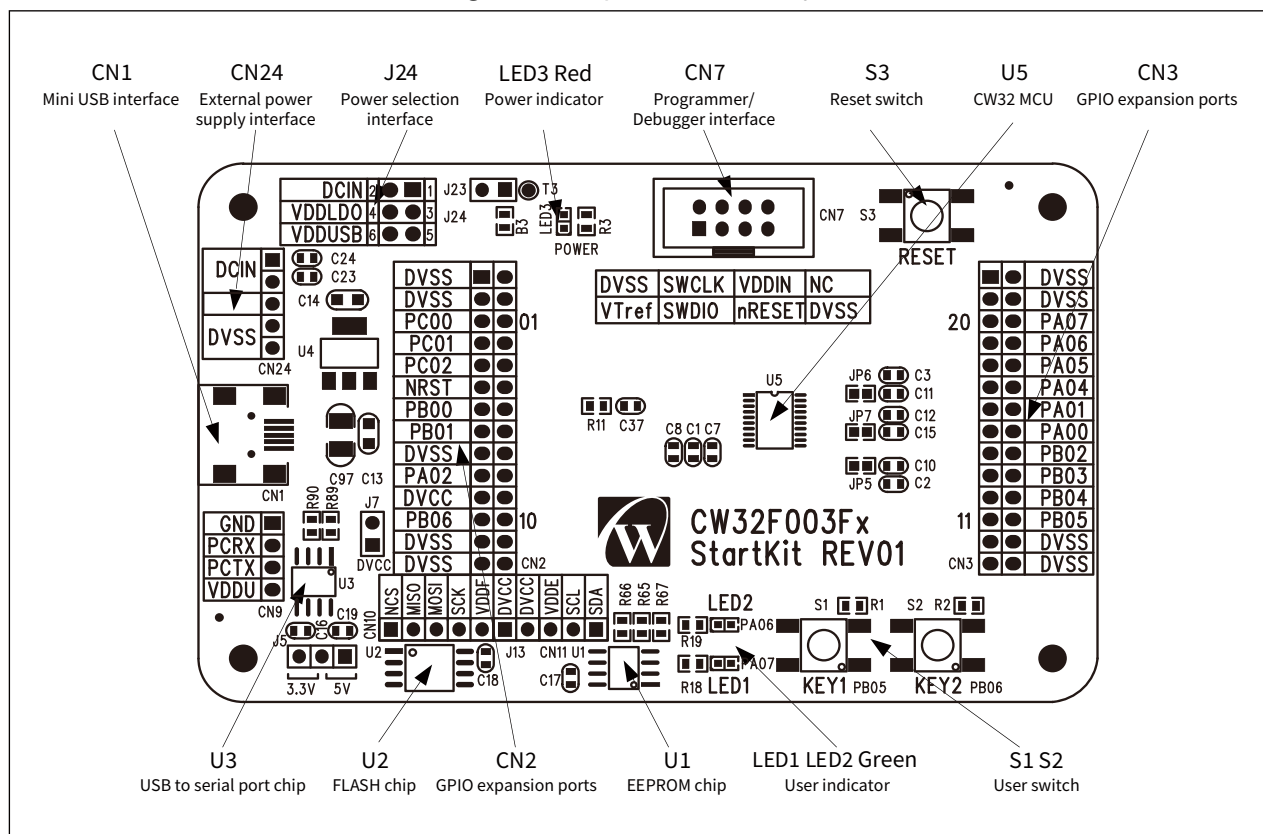
Figure 6-1 Top-level device layout
