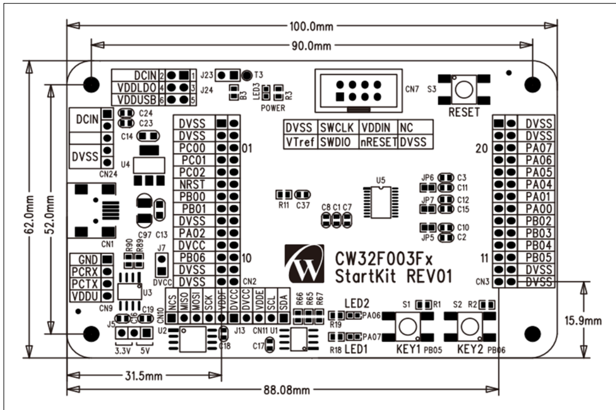
Figure 6-2 CW32F003FxFx StartKit Mechanical Dimensions
